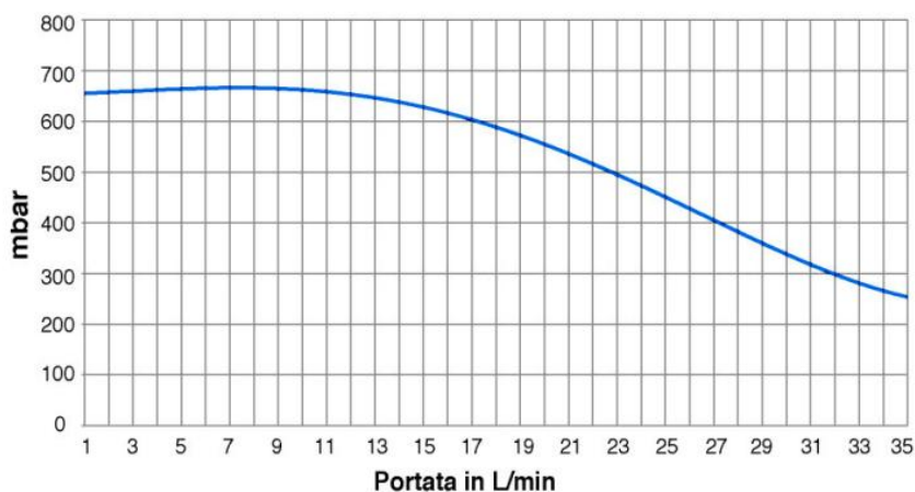
PREVALENZA RESIDUA DN25 MODULANTE / RESIDUAL HEAD DN25 MIXED MOTORIZED GROUP
