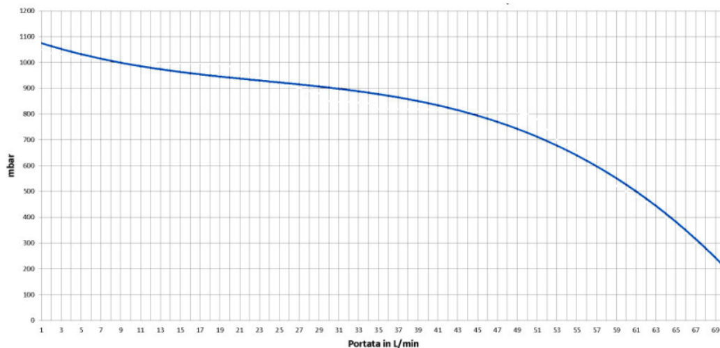
PREVALENZA RESIDUA DN32 MODULANTE / RESIDUAL HEAD DN32 MIXED MOTORIZED GROUP
