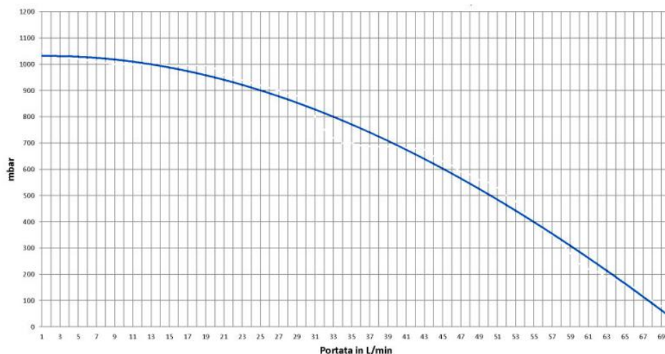
PREVALENZA RESIDUA DN32 PUNTO FISSO / RESIDUAL HEAD DN32 MIXED FIXEDPOINT GROUP
