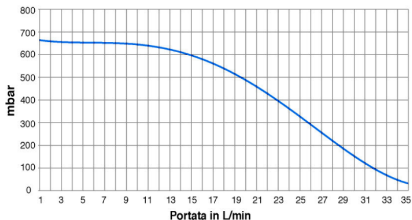
PREVALENZA RESIDUA DN25 PUNTO FISSO / RESIDUAL HEAD DN25 MIXED FIXEDPOINT GROUP
