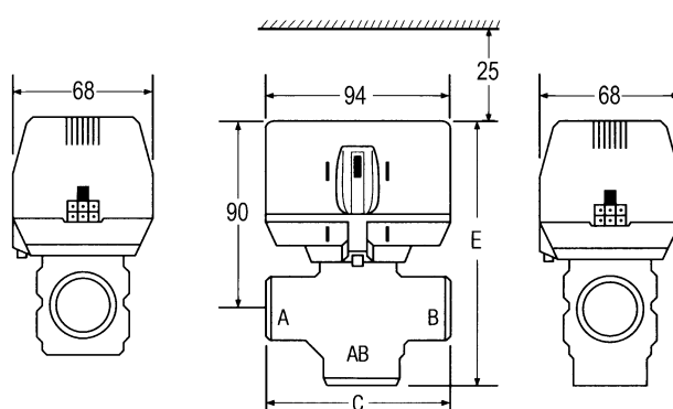
Valvola a 3 vie
